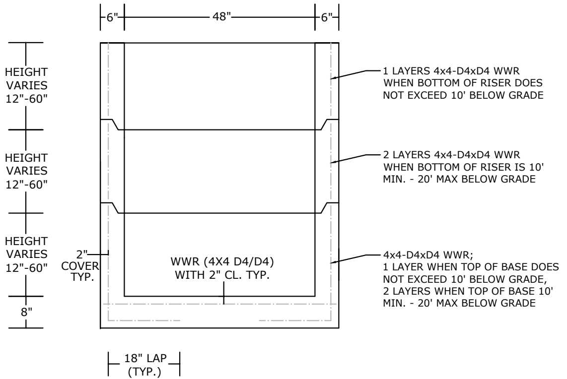
SECTION VIEW
