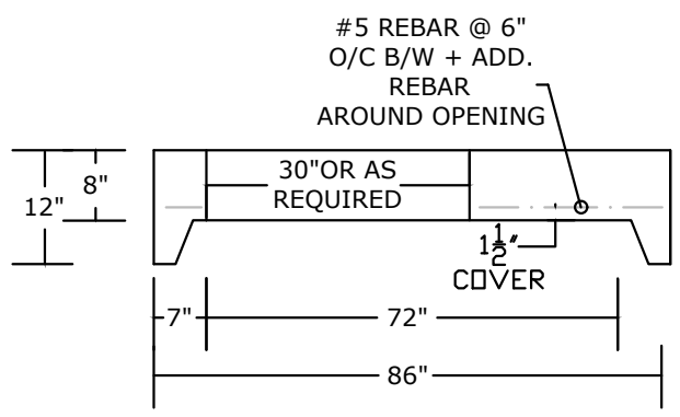
FLAT TOP SIDE VIEW
