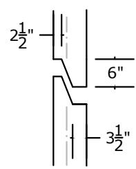
JOINT DETAIL
