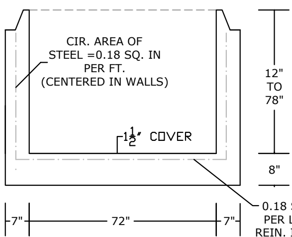
BASE SECTION
