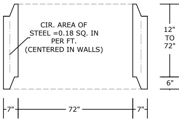
RISER SECTION
