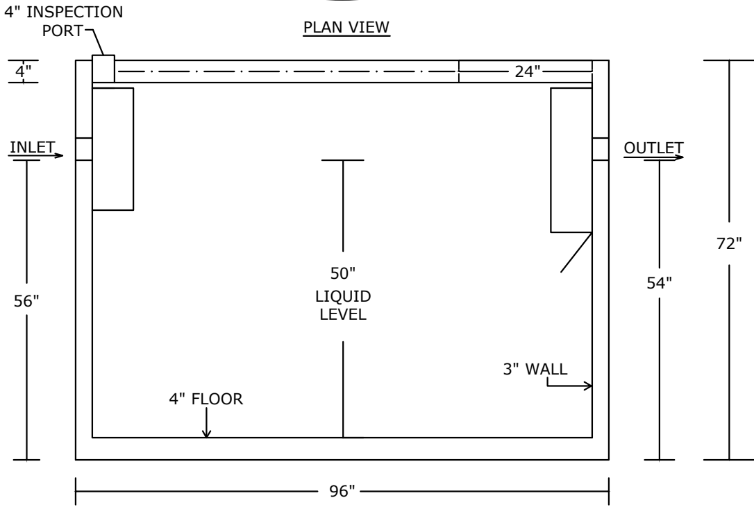
SECTION VIEW
