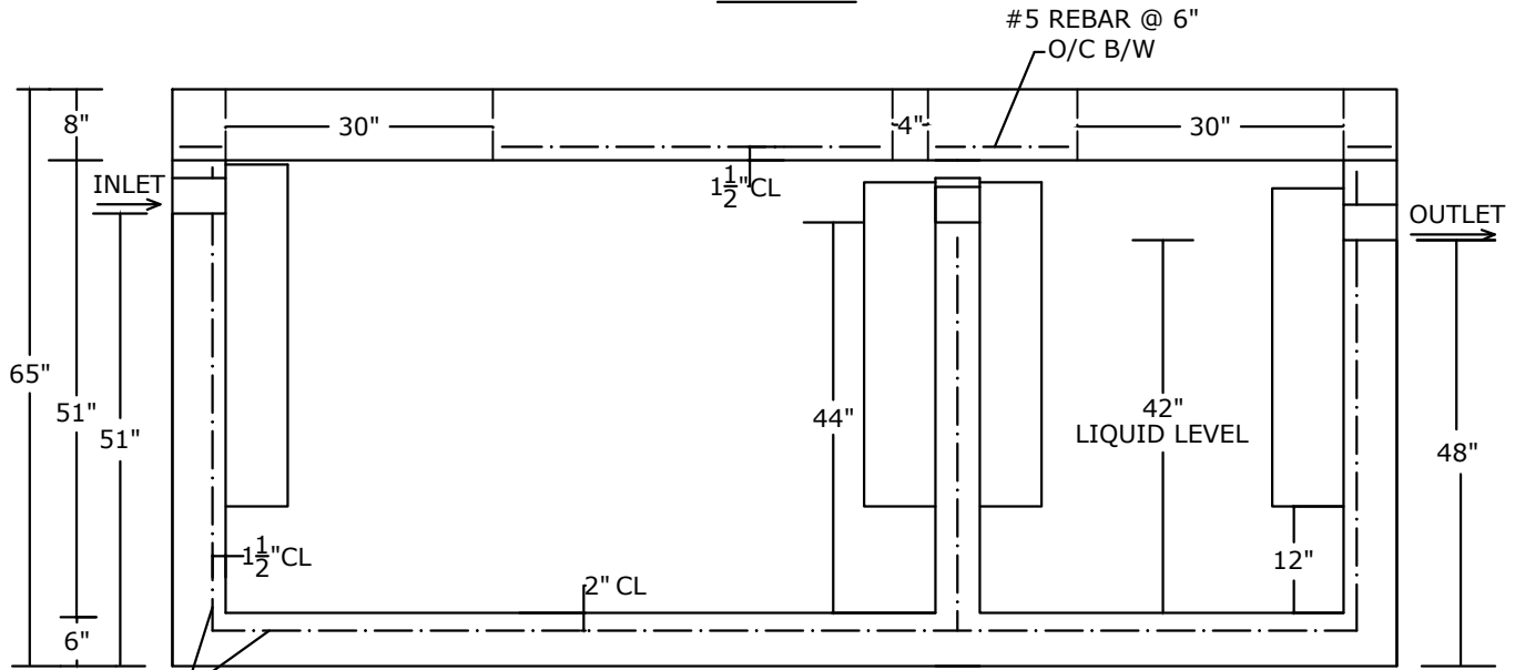
SECTION VIEW
